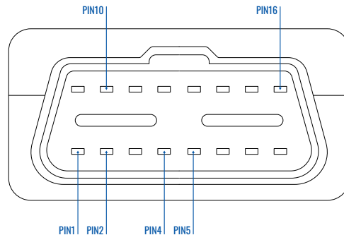
FMB010 OBDII socket pinout
