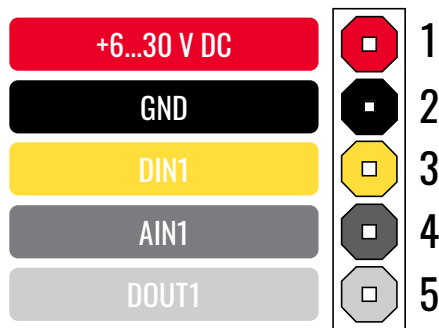
FMB910 pinout
