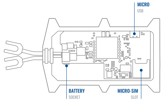
TOP VIEW (WITHOUT COVER)
