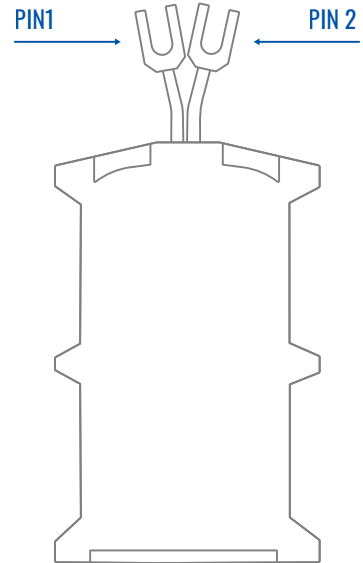
FMC800 socket pinout
