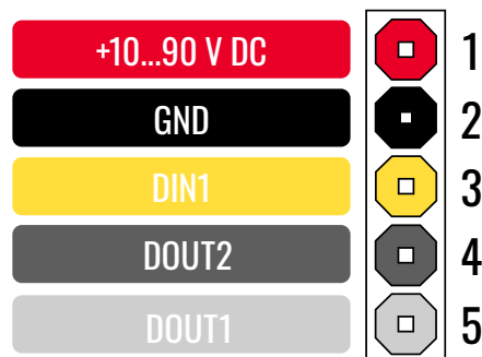
FMB930 pinout
