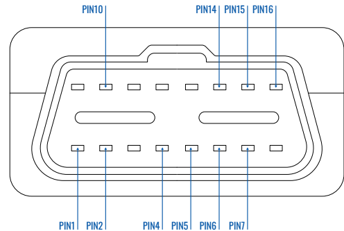
FMB001 OBDII socket pinout
